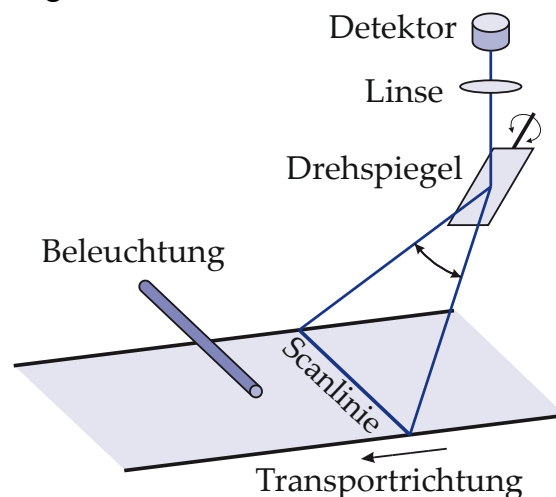
Flying-Image-Scanner
