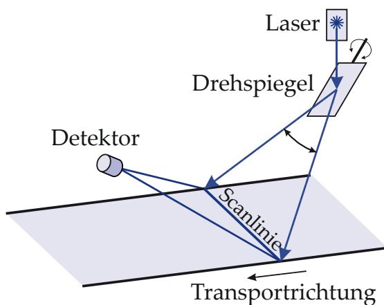
Flying-Spot-Scanner
